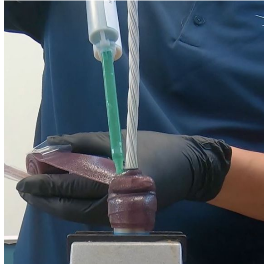
Connector Wrap Installation
